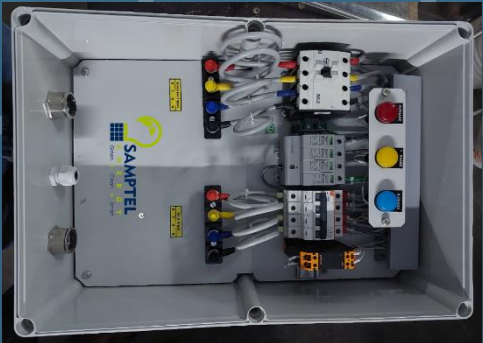
SOLAR ACDB
